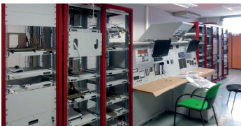
Hardware and software support bench for troubleshooting Overview of the complete bench.
