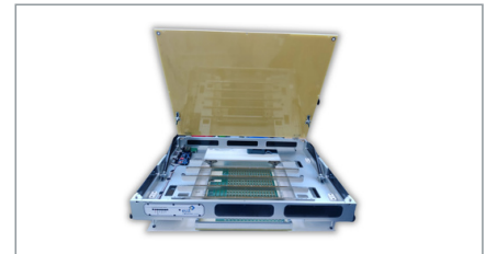
ICT fixture for EIIT XILS-1200 handler
