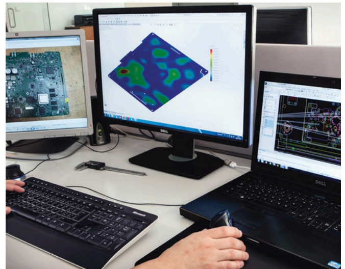
FEA Analysis
