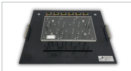
Specific FCT fixture for RU-030 system
