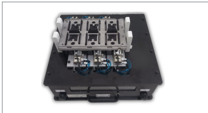
Custom fixture for specific InLine handler
