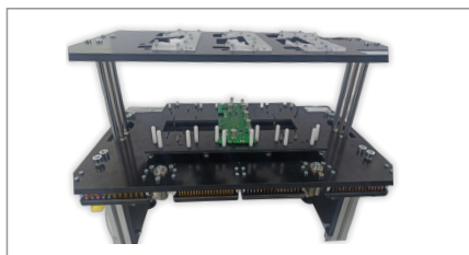
Manual ICT/ISP/FCT fixture for Engmatec system
