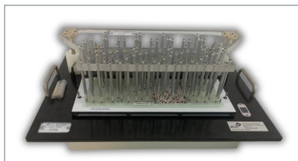
ICT fixture for EIIT RU-100 system
