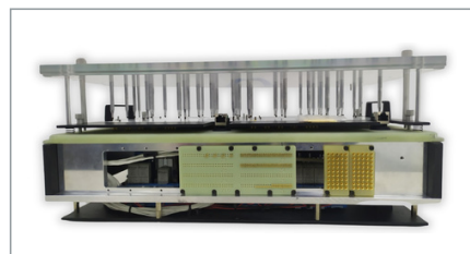
Interchangeable Kit Ingun FCT fixture
